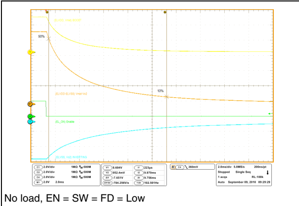
Figure 8. Fast discharge
